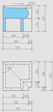
wedi Sanoasa Bellina corner bench element 90°, transition straight
