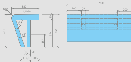
wedi Sanoasa bench 3, 900 mm
