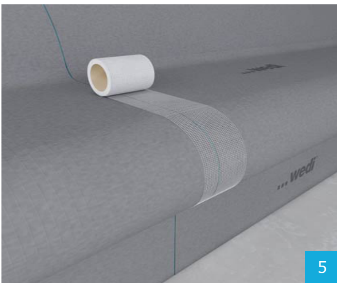
Apply wedi Tools reinforcement tape to all joints of the bench elements.
