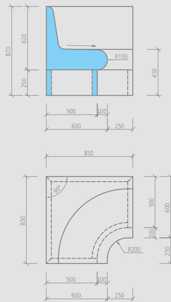
wedi Sanoasa Comoda corner bench element 90°, transition rounded
