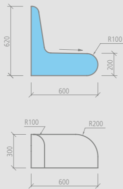
wedi Sanoasa Comoda end bench element left, Corner radius 200 mm
