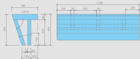
wedi Sanoasa bench 2, 1.200 mm
