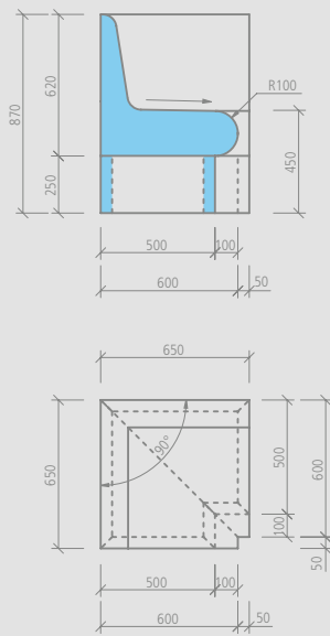
wedi Sanoasa Comoda corner bench element 90°, transition straight
