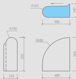
wedi Sanoasa Bellina end bench element right, Corner radius 486 mm
