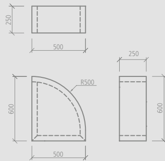
wedi Sanoasa Comoda end base element, Corner radius 600 mm
