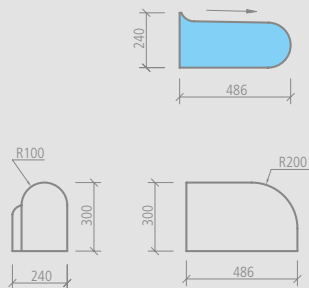
wedi Sanoasa Bellina end bench element left, Corner radius 200 mm
