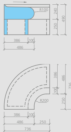
wedi Sanoasa Bellina corner bench element 90°, transition rounded
