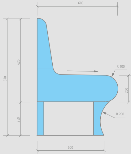
wedi Sanoasa Comoda bench element, finish round
