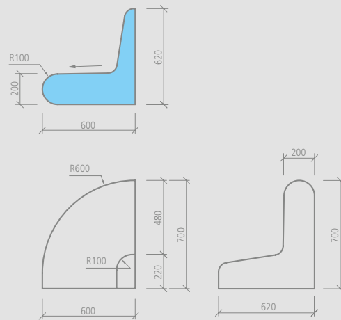
wedi Sanoasa Comoda end bench element right, Corner radius 600 mm
