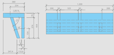
wedi Sanoasa bench 1, 1.200 mm
