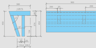
wedi Sanoasa bench 2, 900 mm
