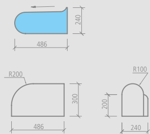
wedi Sanoasa Bellina end bench element right, Corner radius 200 mm
