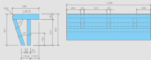
wedi Sanoasa bench 3, 1.200 mm
