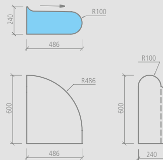
wedi Sanoasa Bellina end bench element left, Corner radius 486 mm
