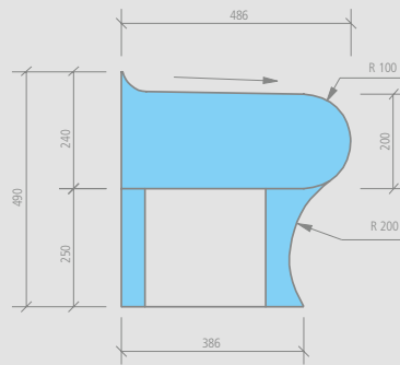
wedi Sanoasa Bellina bench element, finish length round
