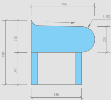
wedi Sanoasa Bellina bench element, finish length straight
