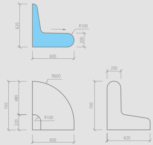
wedi Sanoasa Comoda end bench element left, Corner radius 600 mm
