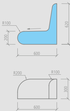
wedi Sanoasa Comoda end bench element right, Corner radius 200 mm
