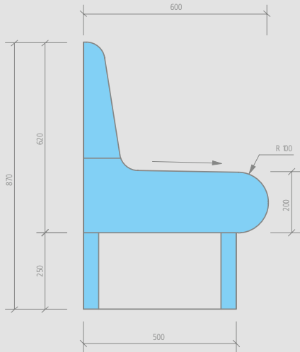
wedi Sanoasa Comoda bench element, finish straight
